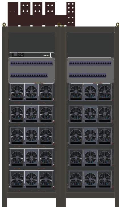
168KW POWER CABINET WITH 5.6 KW CENTRIX RECTIFIERS
